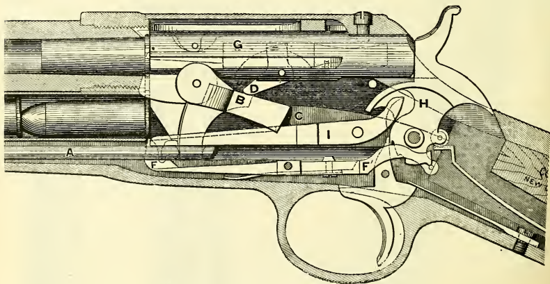
Mechanism of the Colt "Lightning" Rifle.
